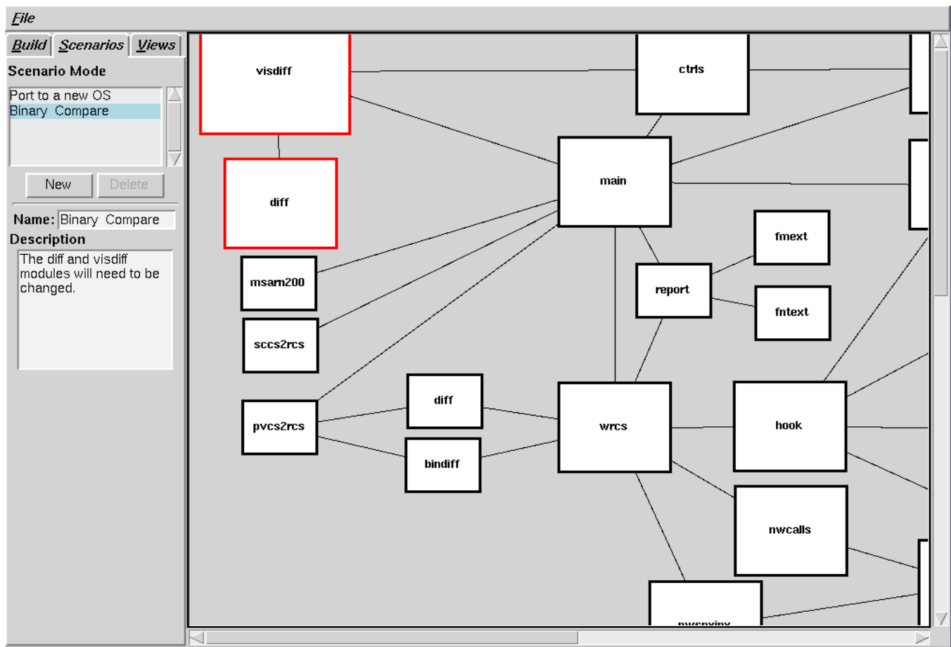
Figure 1: A Fish-eye View of an Architecture in SAAMtool
