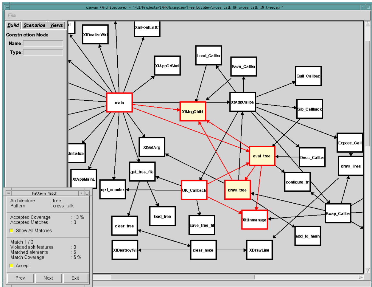
Figure 2: An Example of Architectural Pattern Matching in SAAMtool
