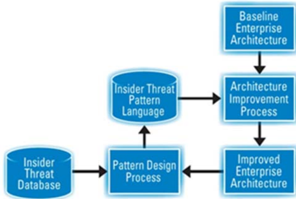
Figure 1: Approach to Developing an Insider Threat Enterprise Architectural Pattern Library
