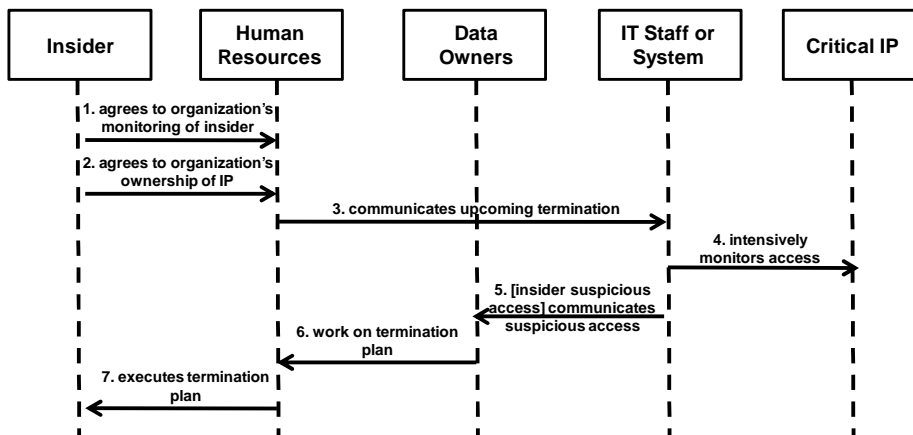
Figure 2: Sequence Diagram for Increased Monitoring of Departing Insiders
