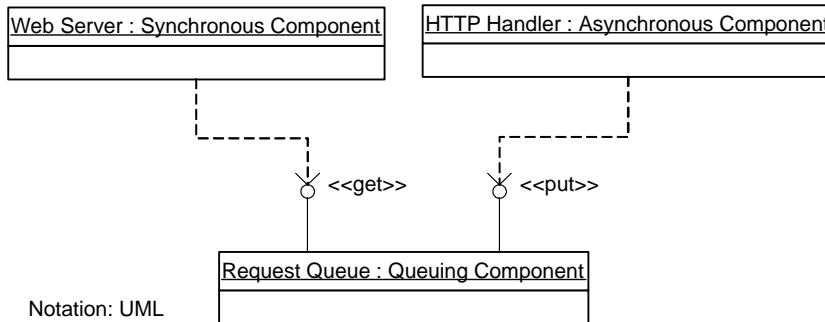
Figure 11: Half-Sync/Half-Async Pattern Applied in the JAWS
