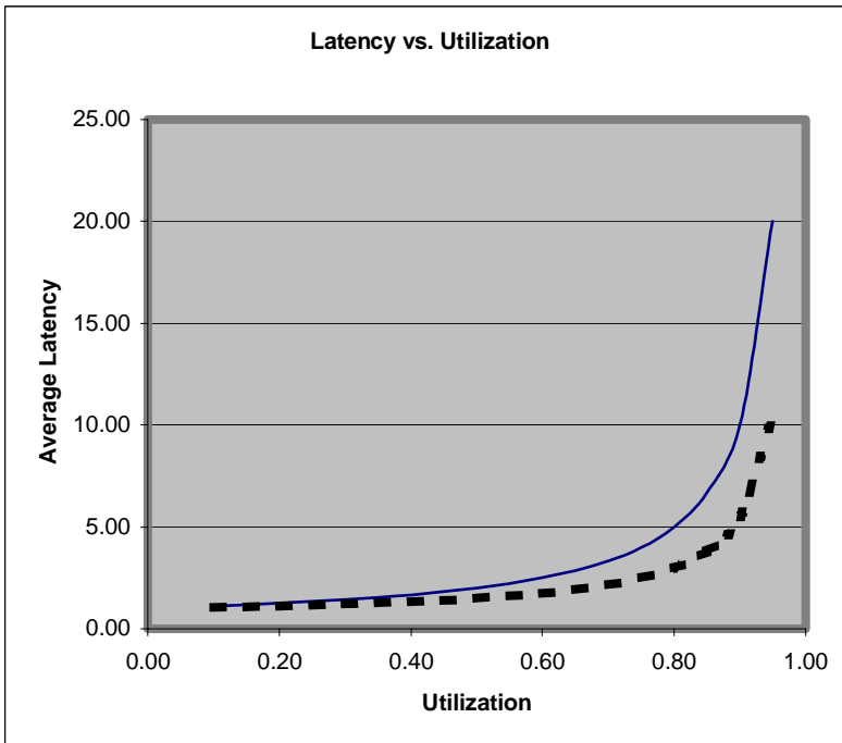
Figure 18: Graph Showing Average Latency as a Function of Utilization for Constant and Exponential Execution Times When the Average Execution Time is 1 ms
