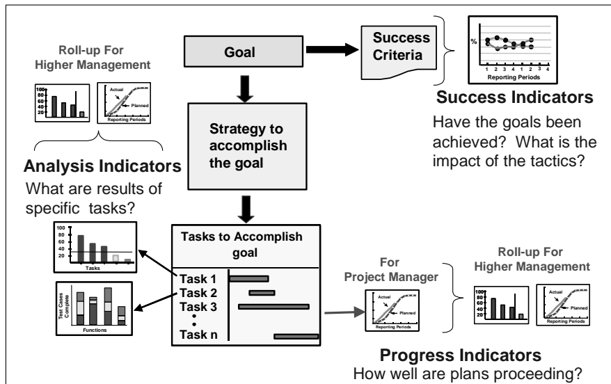
Figure 3: Indicator Classification
