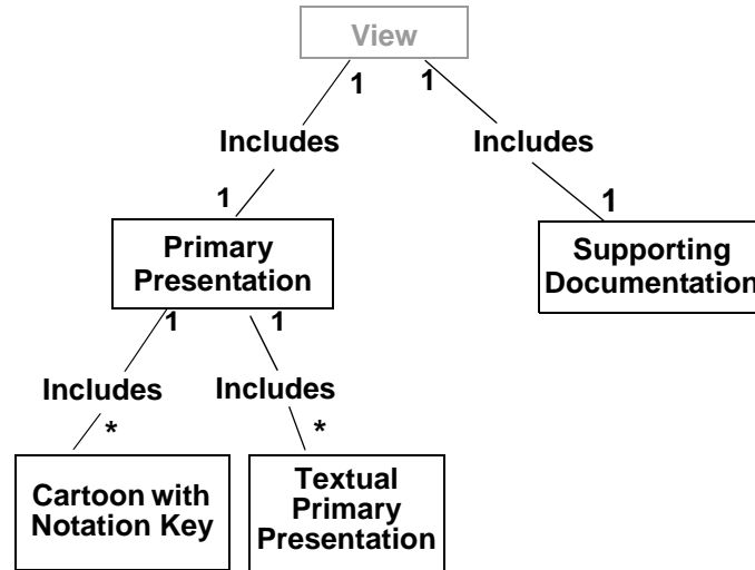
Figure 2: View Is Documented By a Primary Presentation and Supporting Documentation
