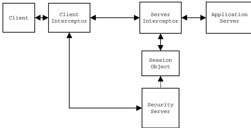
Figure 1. Secured Application Using Sorbet
