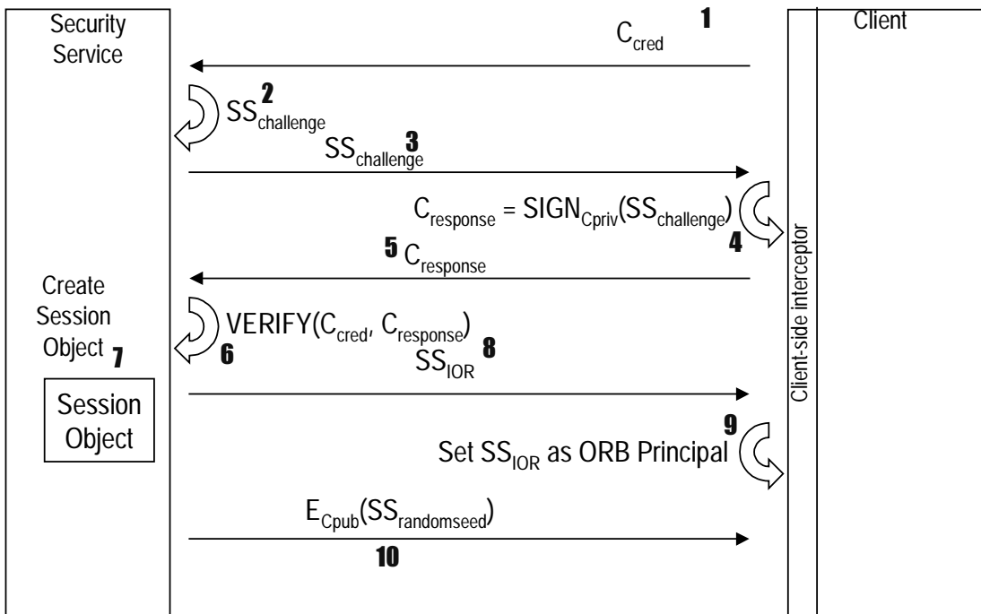
Figure 2. Client Authentication
