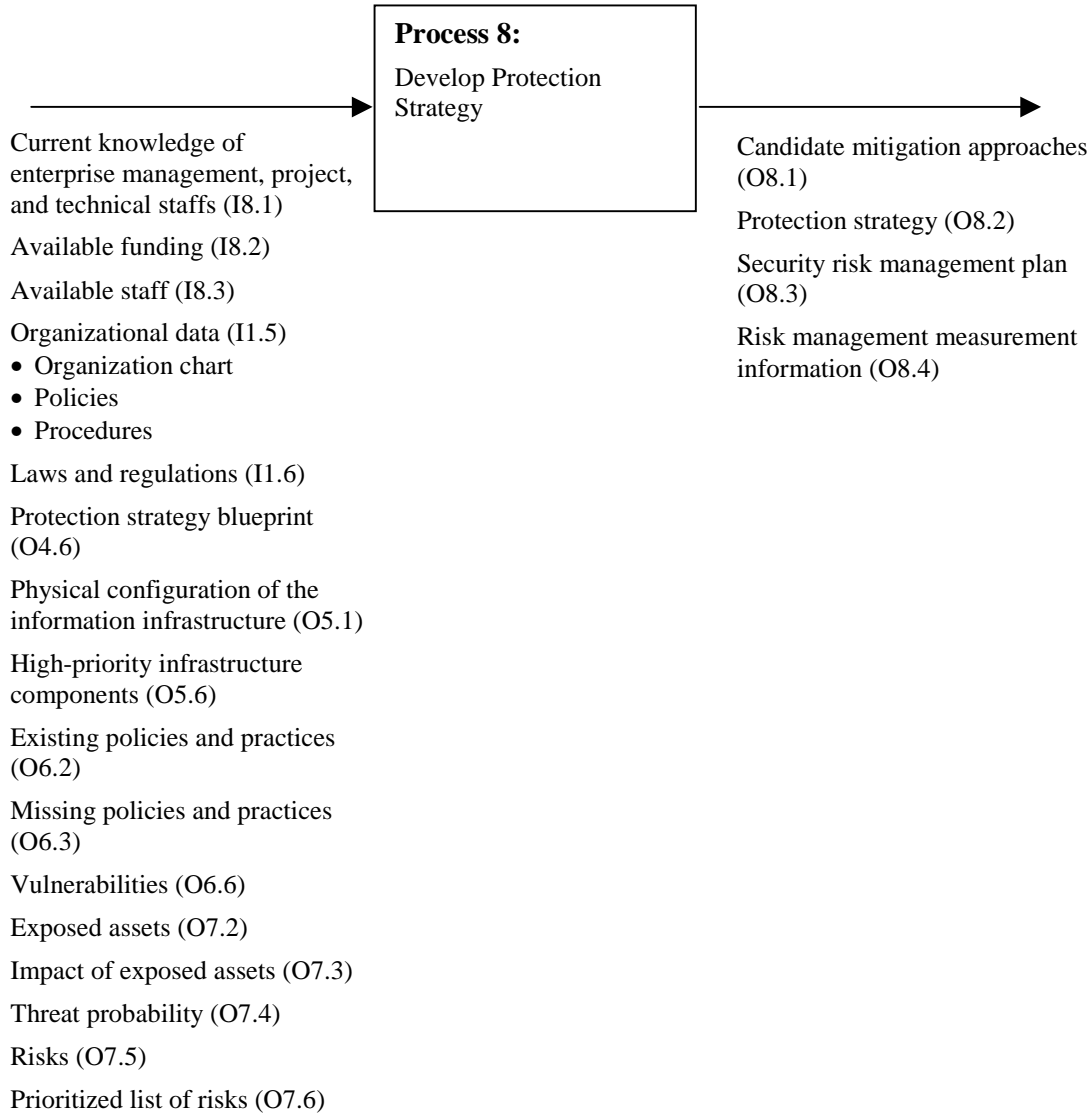
Figure 11: OCTAVE Process 8, Develop Protection Strategy
